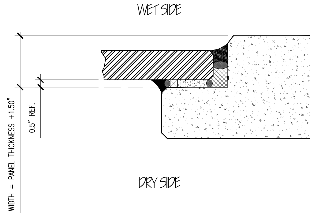
1A TYPICAL JAMB INSTALLATION DETAIL SCALE: NOT TO SCALE
