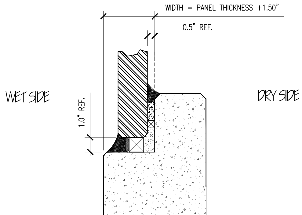
8A TYPICAL SILL INSTALLATION DETAIL SCALE: NOT TO SCALE
